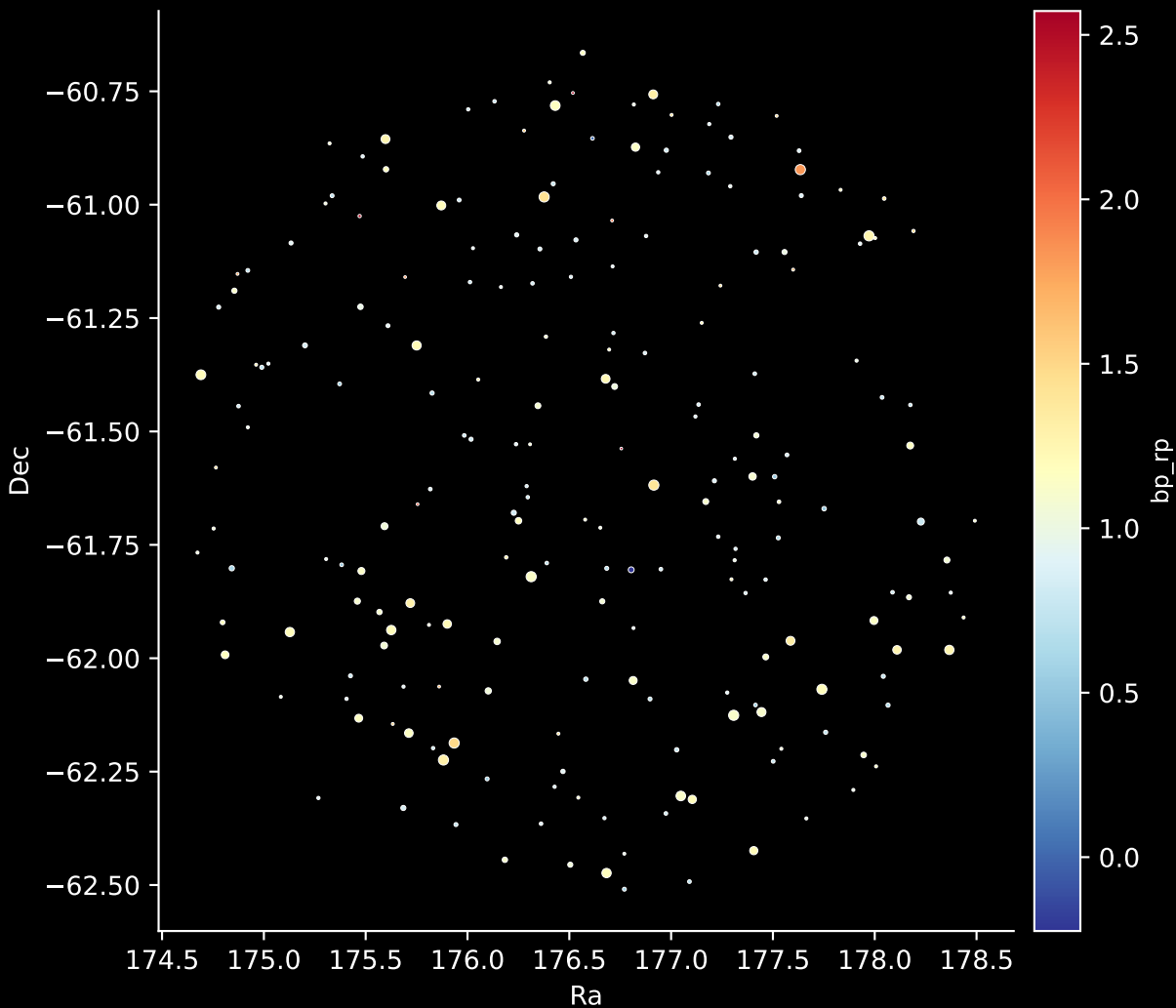
APOGEE DR17 Field: [271-36-O_TESS] Stars: 208
