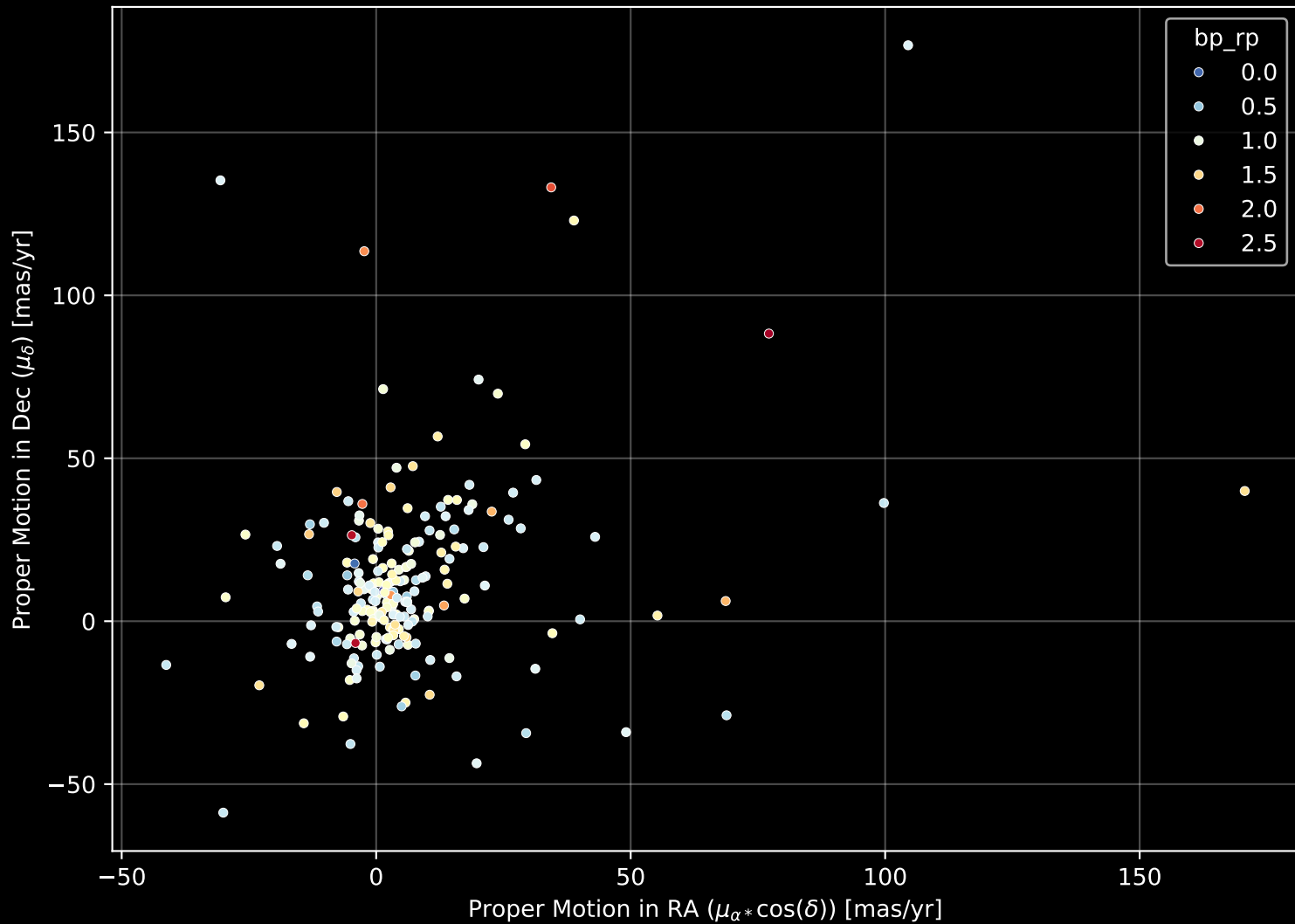
APOGEE DR17 Field: [271-36-O_TESS] Proper Motion Diagram (n= 208)
