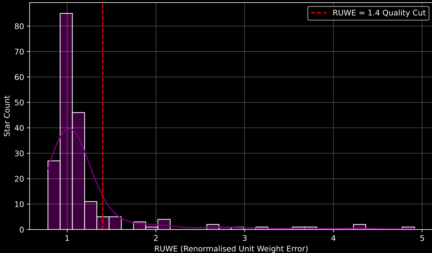
GAPOGEE DR17 Field [271-36-O_TESS] RUWE Distribution (n= 197)
