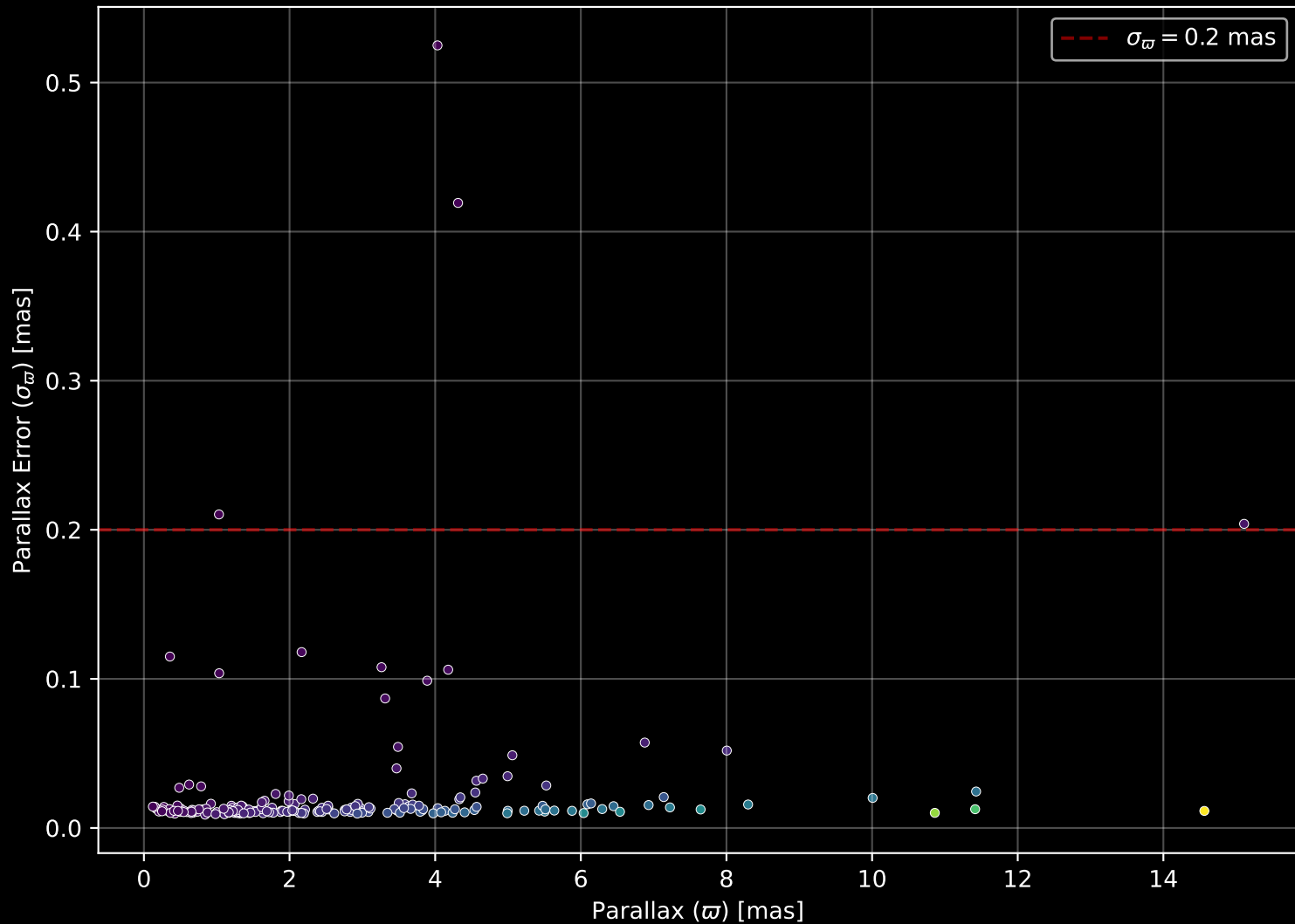
APOGEE DR17 Field: [271-36-O_TESS] Parallax Quality (n= 208)
