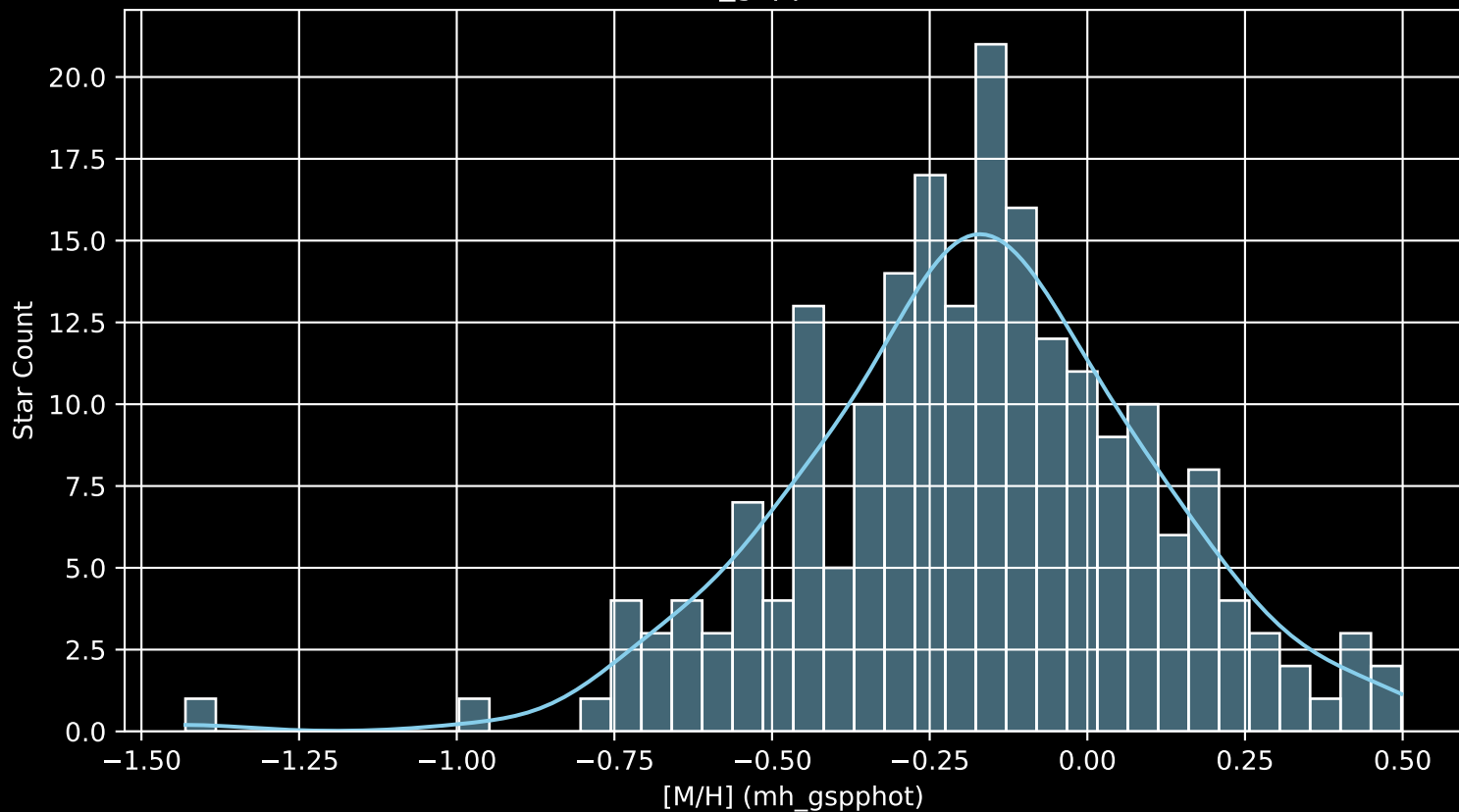
APOGEE DR17 Field: [271-36-O_TESS [M/H] (mh_gspphot) (n= 208)
