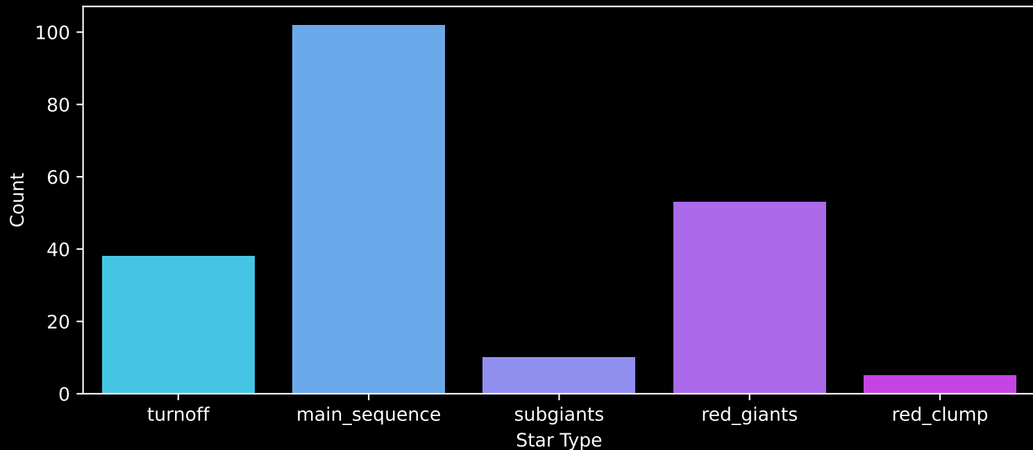
APOGEE DR17 Field: [271-36-O_TESS] Count plot of Star Type
